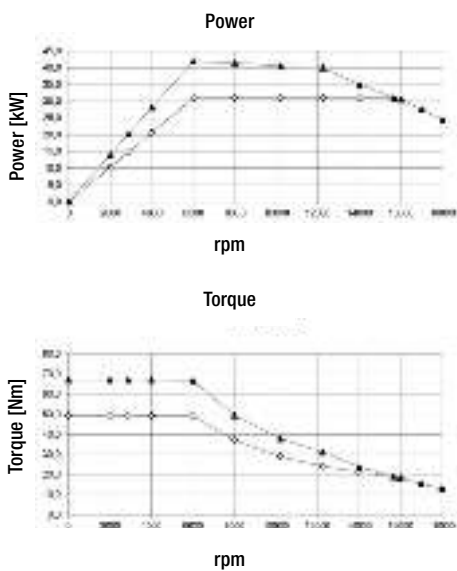
Motor spindle type 1
