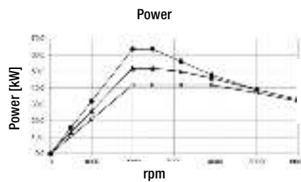
Motor spindle – draw-bar spindle type 10
